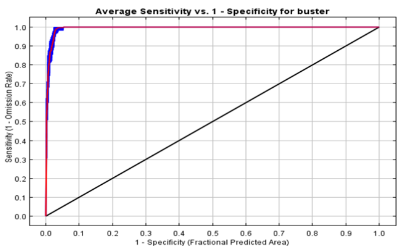
Figure 7: Receiver Operating Characteristic (ROC) curve generated by the MaxEnt model
